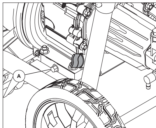
Figure 32 – Oil Drain Plug
