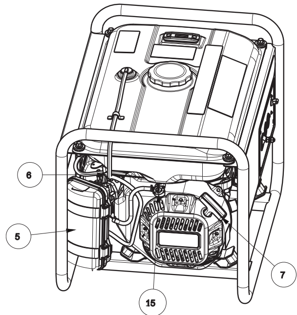
Figure 3 - Generator/Engine Controls
