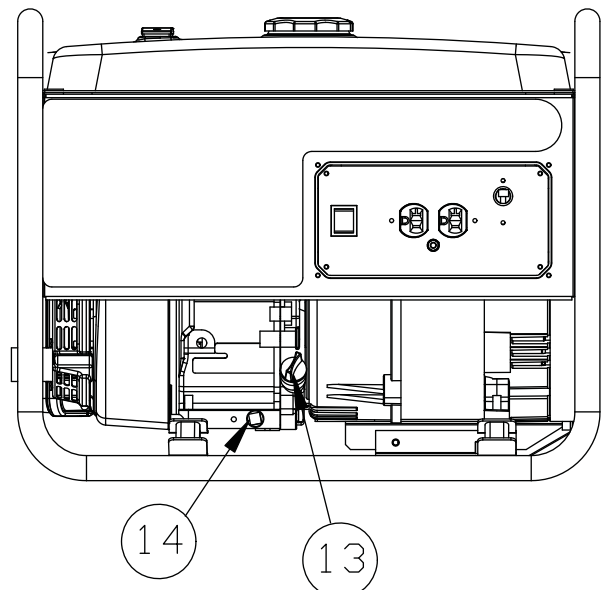
Figure 3 - Generator/Engine Controls
