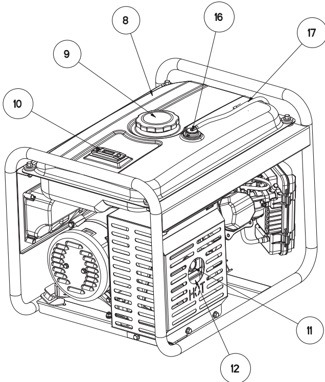
Figure 4 - Silencieux
