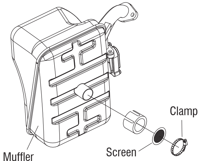
Figure 9 - Spark Arrestor
