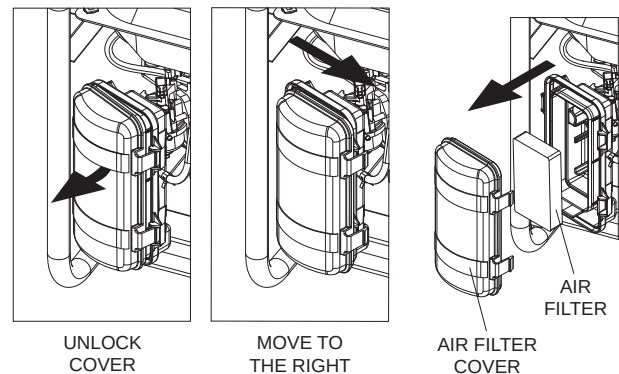
Figure 10 - Air Filter
